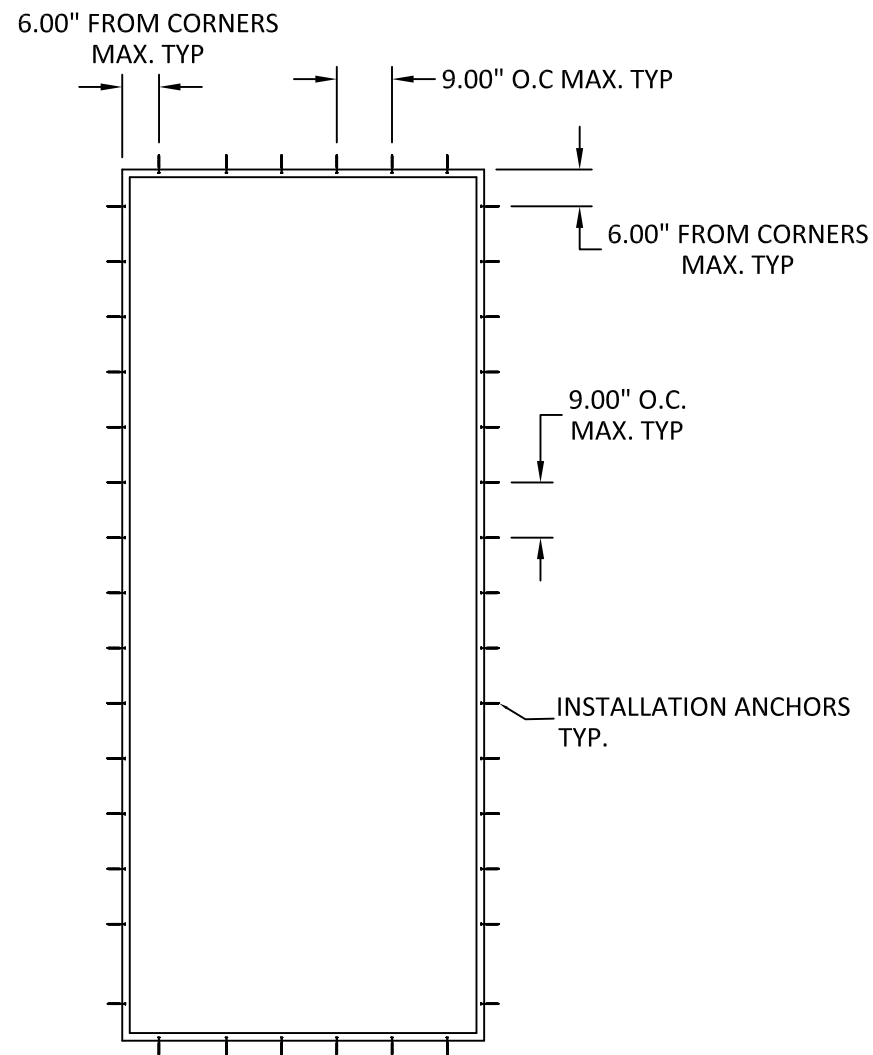
ALUMINUM TUBE TO SUBSTRATE/WALL ANCHORING EXTERIOR ELEVATION
